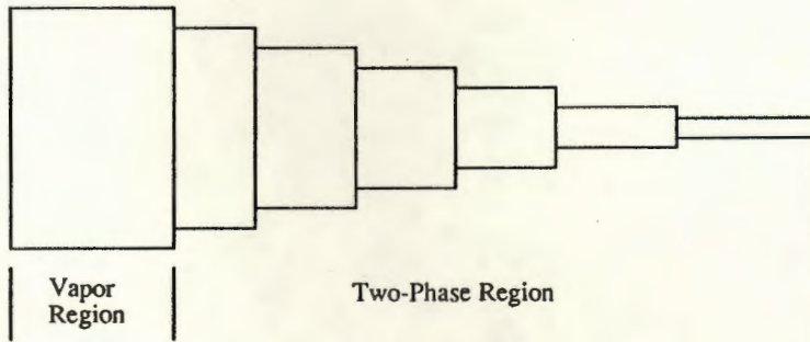
Figure 2. Stepped tube acoustic model for the condenser.
