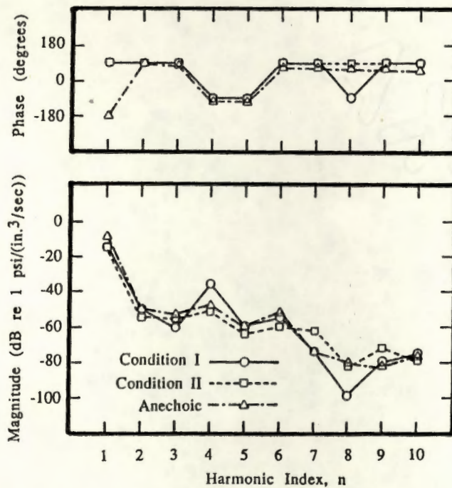
Figure 5. Valve chamber to discharge line acoustic impedance for systems with mufflers.
