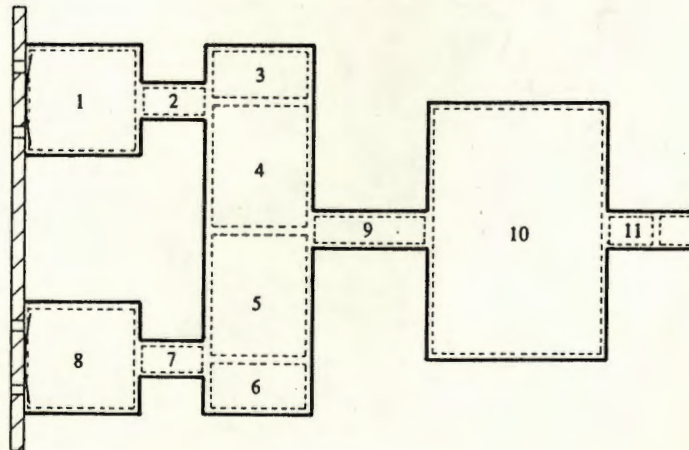
Figure 3. Compressor discharge system acoustic model.
