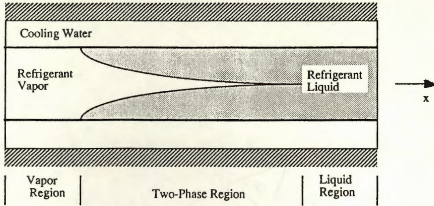
Figure 1. Water cooled, concentric tube heat exchanger.
